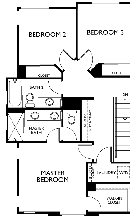
THIRD FLOOR
